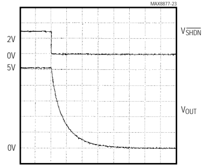
500µs/div MAX8878, NO LOAD
