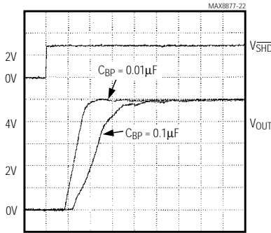
5µs/div MAX887_EUK50, I_{LOAD} = 50mA
