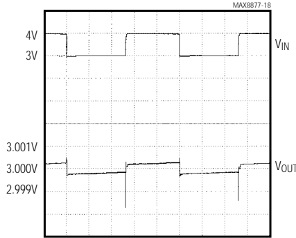
100µs/div MAX887_EUK30, I_{LOAD} = 50mA
