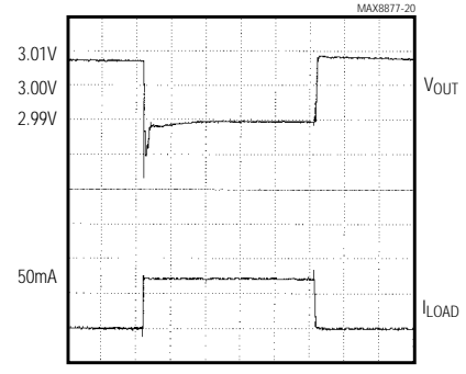
10µs/div MAX887_EUK30, V_{IN} = V_{OUT} + 0.1V , C_{IN} = 10\mu F , I_{LOAD} = 0mA TO 50mA
