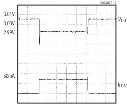
10µs/div MAX887_EUK30, V_{IN} = V_{OUT} + 0.5V , C_{IN} = 10\mu F , I_{LOAD} = 0mA TO 50mA
