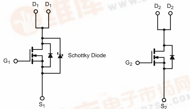
N-Channel MOSFET
