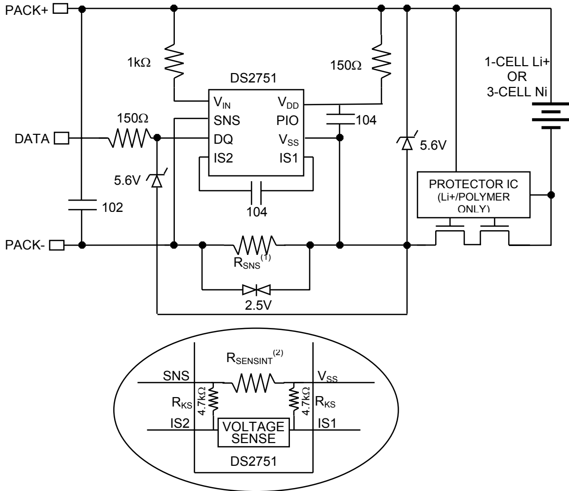
Figure 2. APPLICATION EXAMPLE
