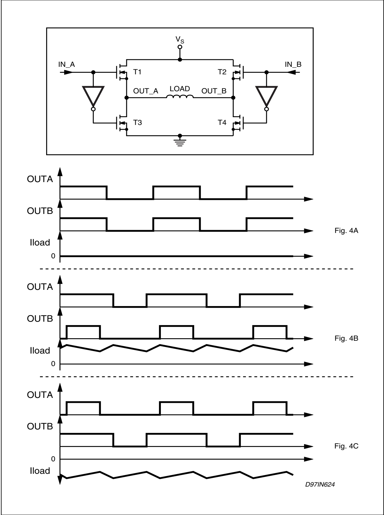
Figure 4. Power Bridge Configuration
