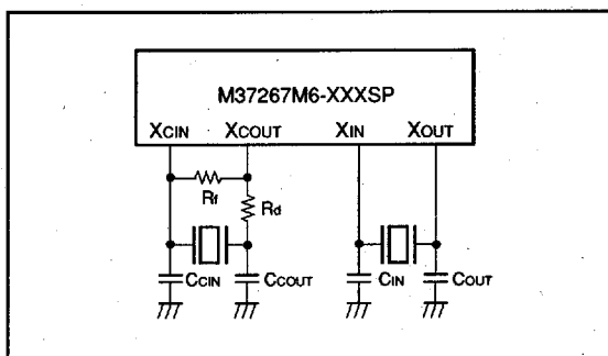
Fig. 85. Ceramic resonator circuit example
