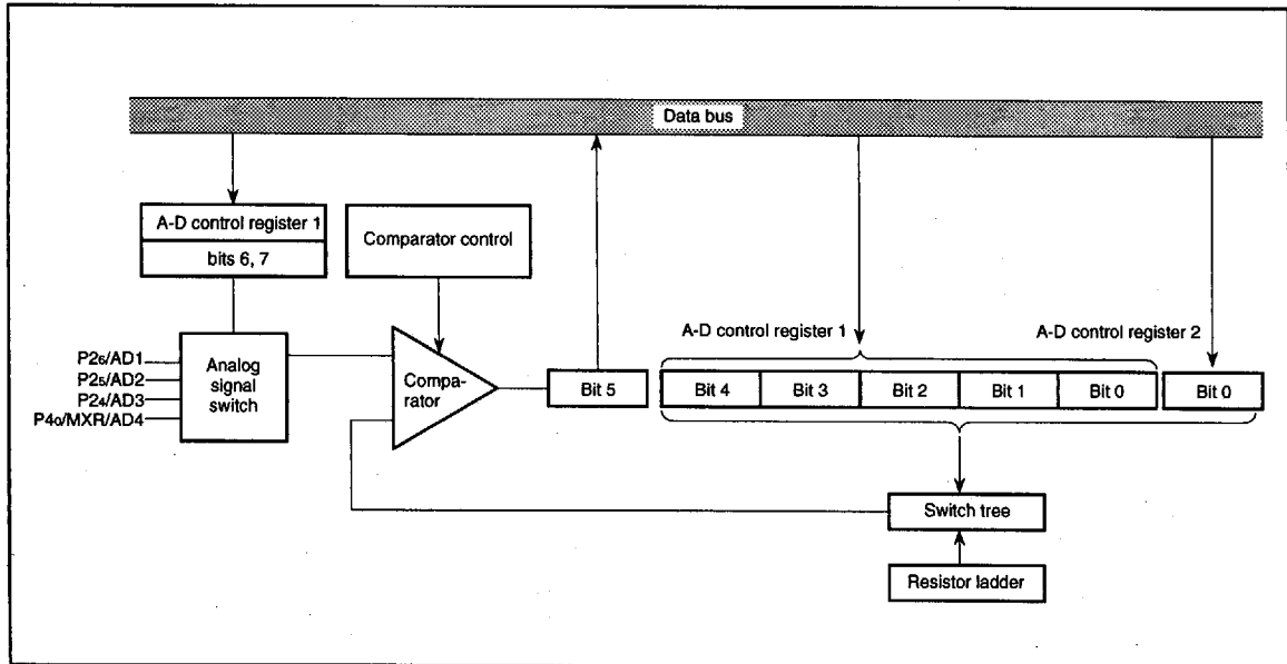
Fig. 17. A-D comparator block diagram
