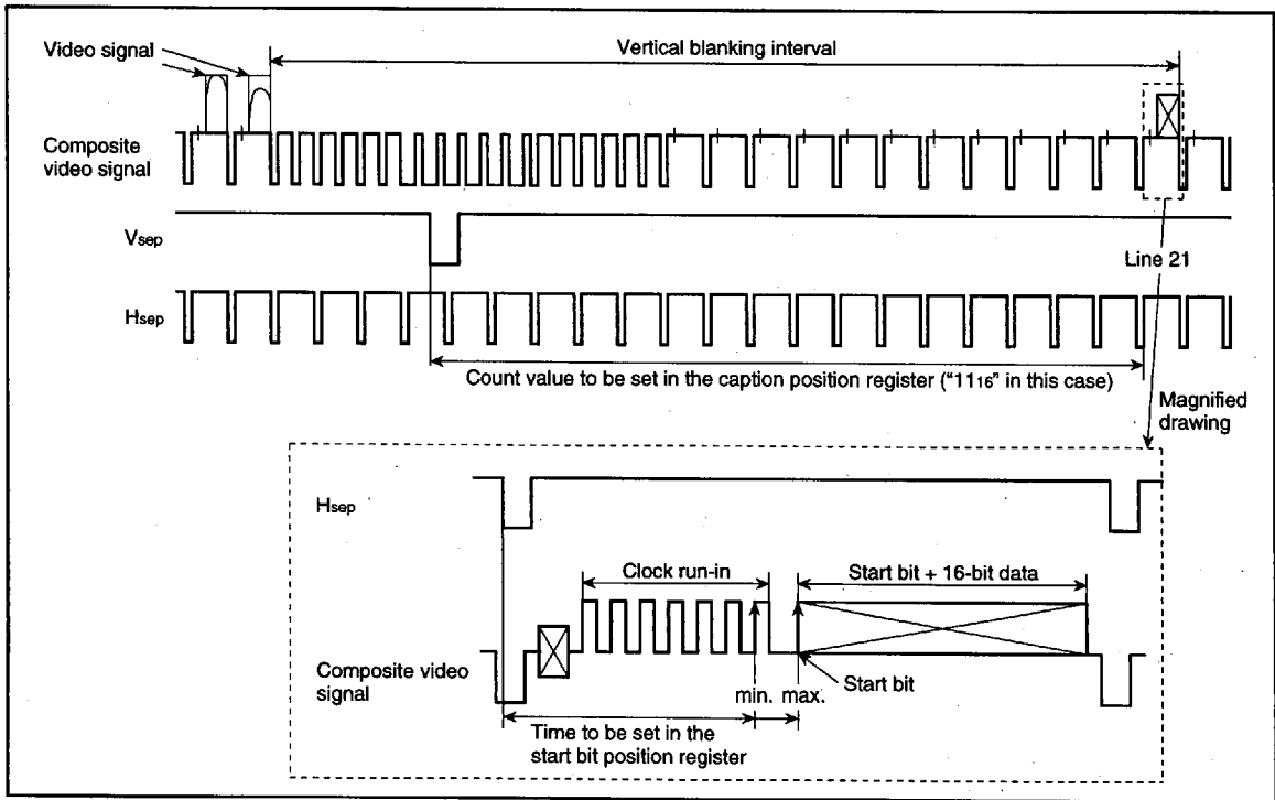
Fig. 23. Signals in vertical blanking interval
