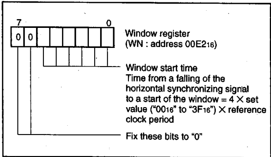
Fig. 28. Structure of window register
