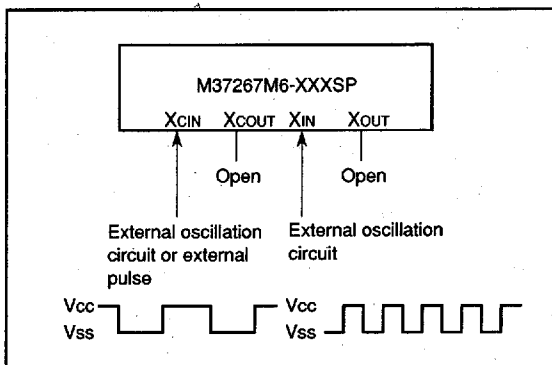
Fig. 86. External clock input circuit example
