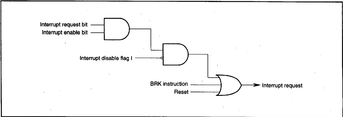
Fig. 6. Interrupt control
