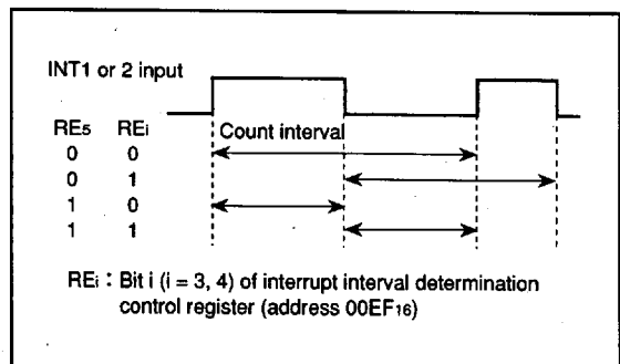
Fig. 79. Setting value of interrupt interval determination control register and measuring interval
