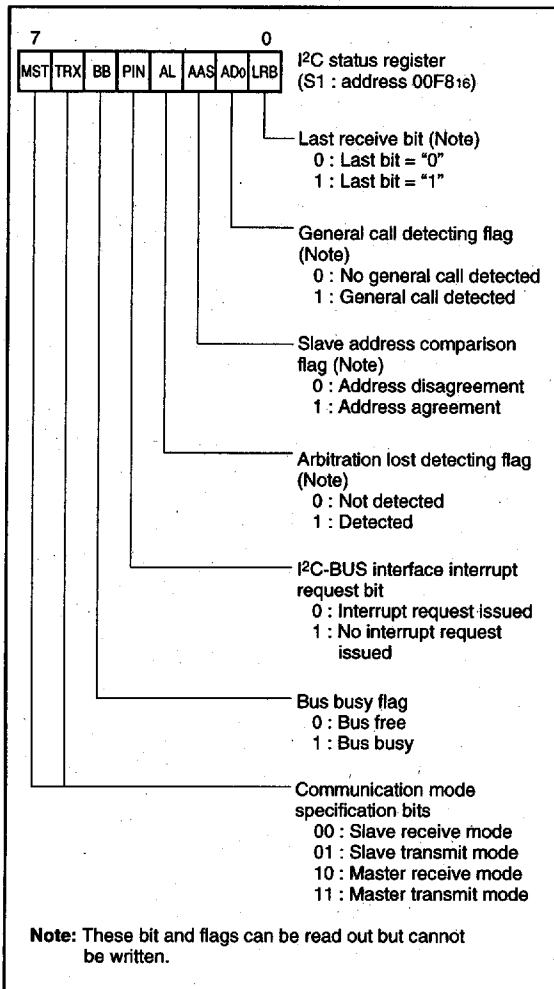
Fig. 39. Structure of I²C status register
