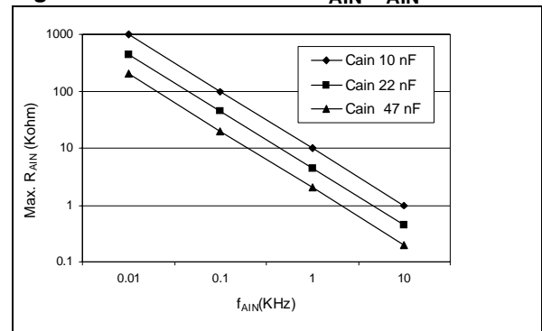
Figure 87. Recommended C_{\text{AIN}}/R_{\text{AIN}} values 4)
