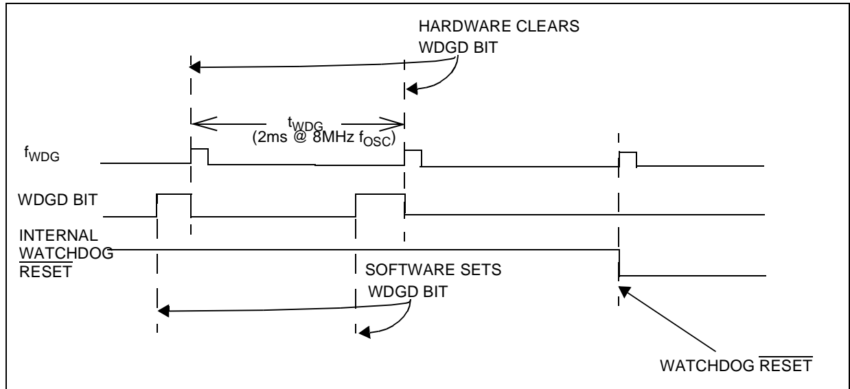
Figure 31. Watchdog Timing Diagram
