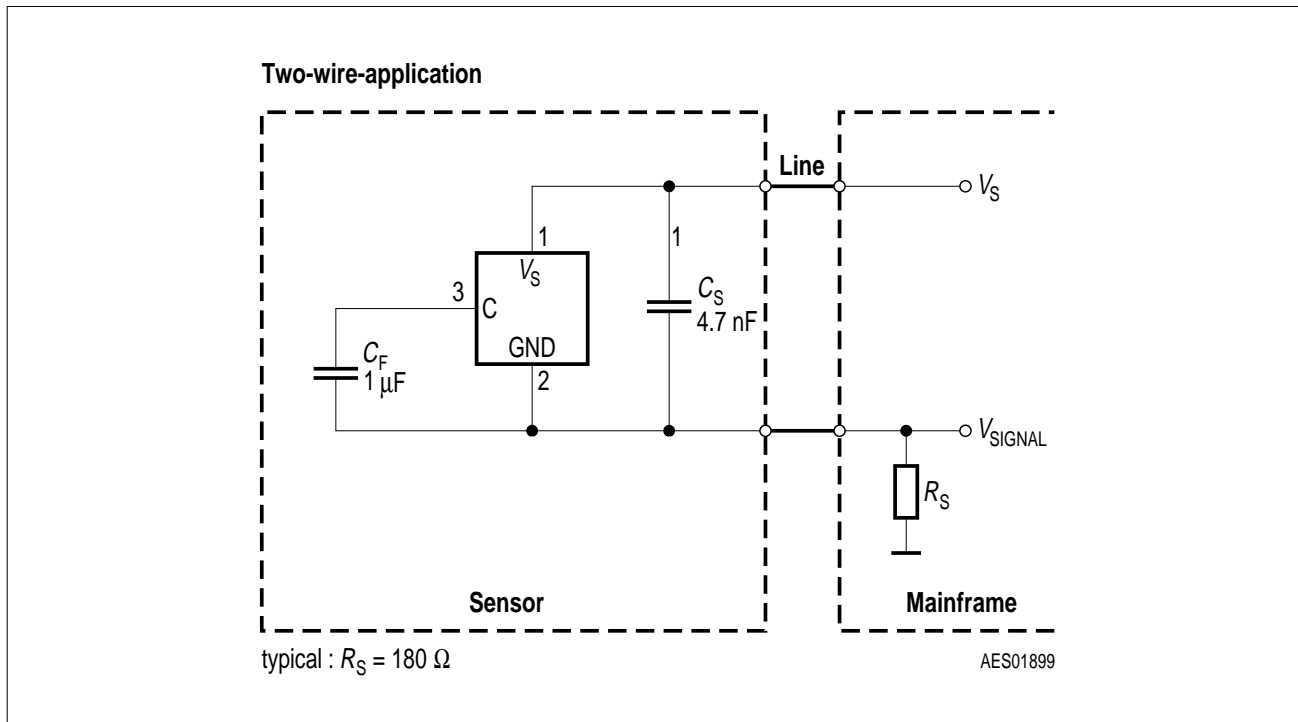
Figure 12 Application Circuit
