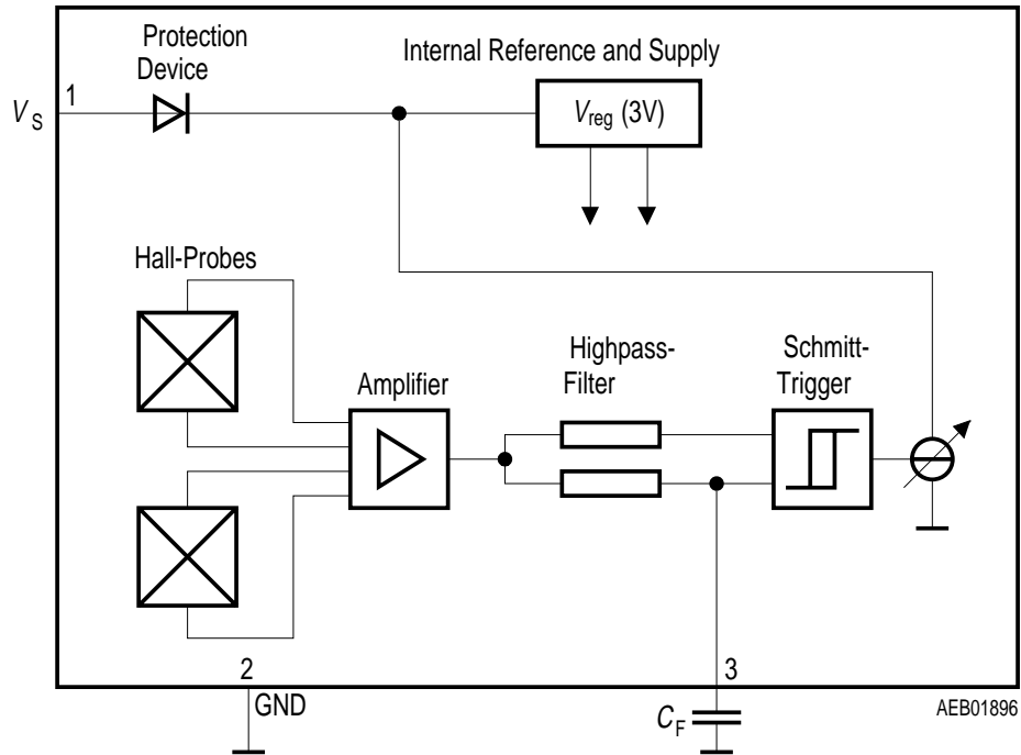
Figure 2 Block Diagram
