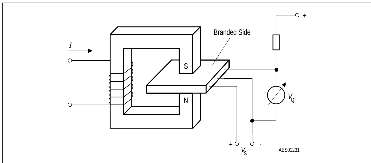
Figure 5 Sensor/Magnetic-Field Configuration
