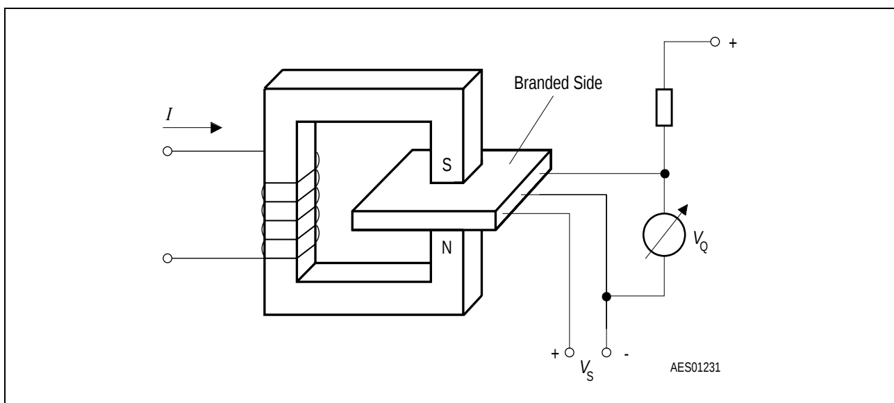
Figure 3 Sensor/Magnetic-Field Configuration
