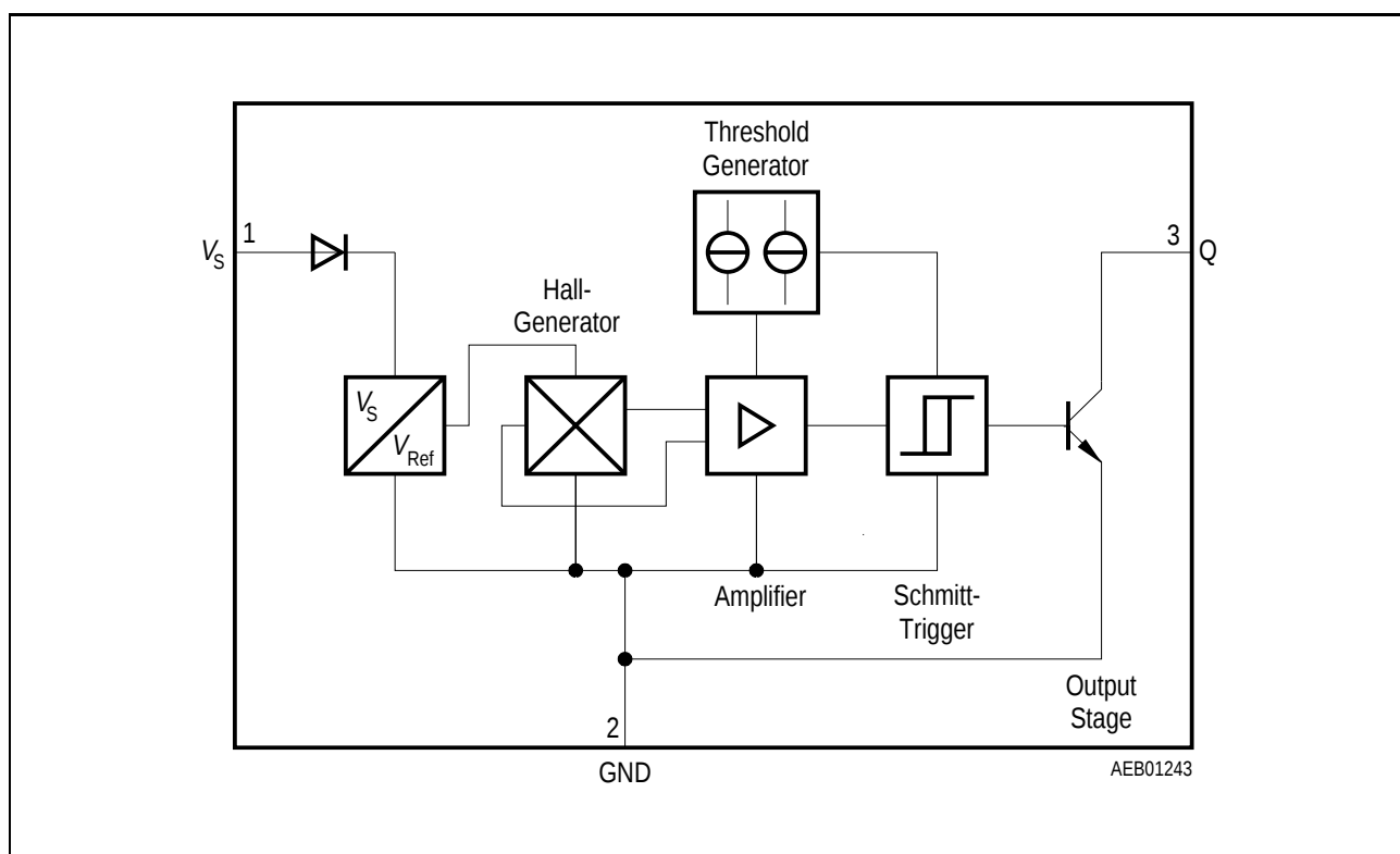
Figure 2 Block Diagram
