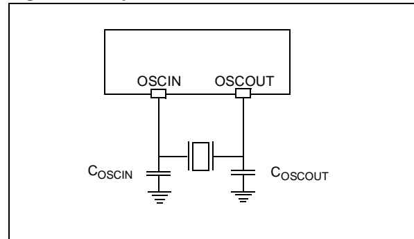
Figure 12. Crystal Resonator
