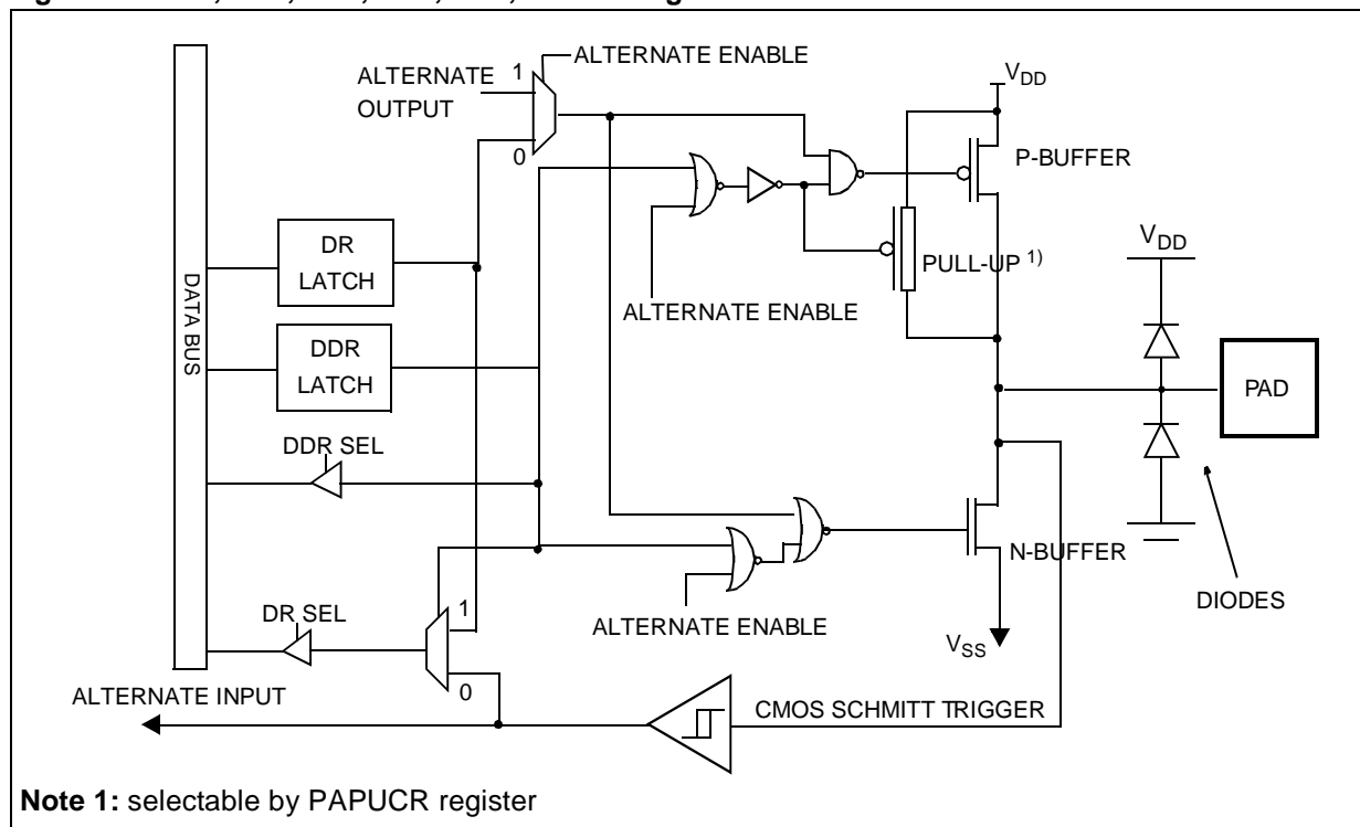
Figure 22. PA6 Configuration
