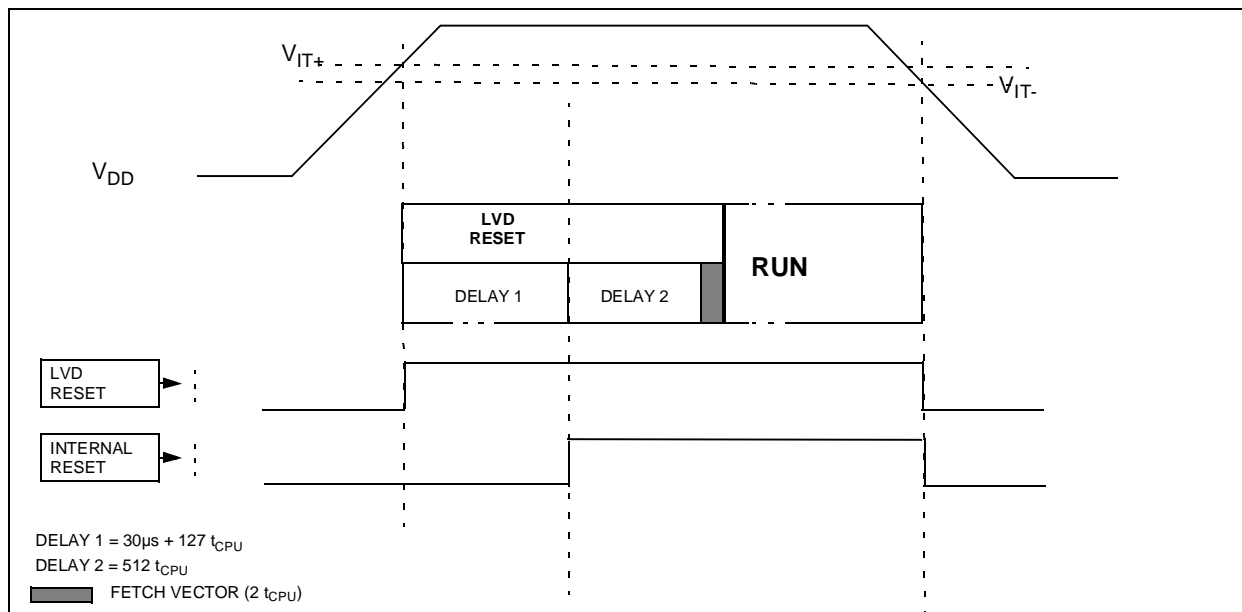
Figure 13. LVD RESET Sequence
