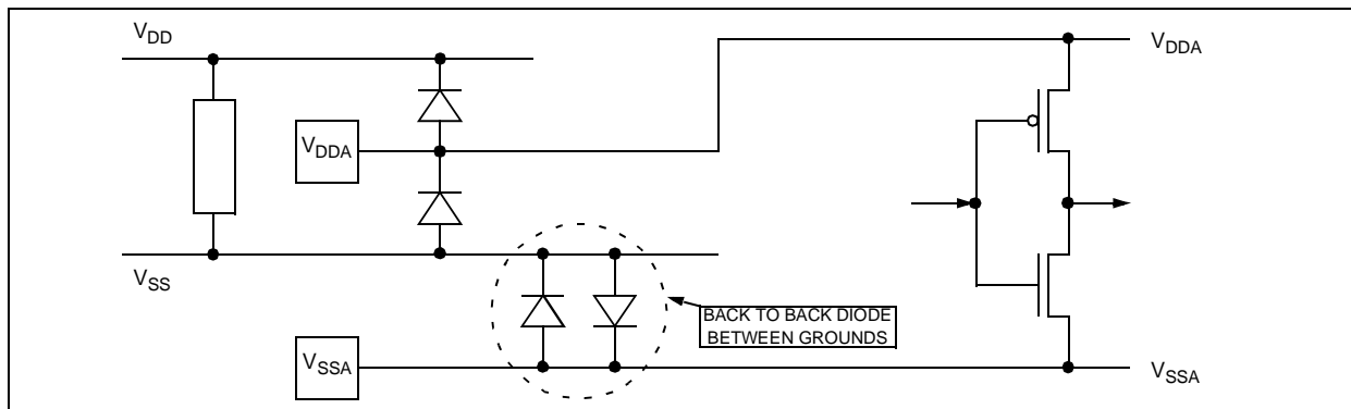
Figure 44. Multisupply Configuration
