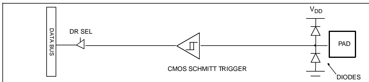
Figure 22. PA6 Configuration
