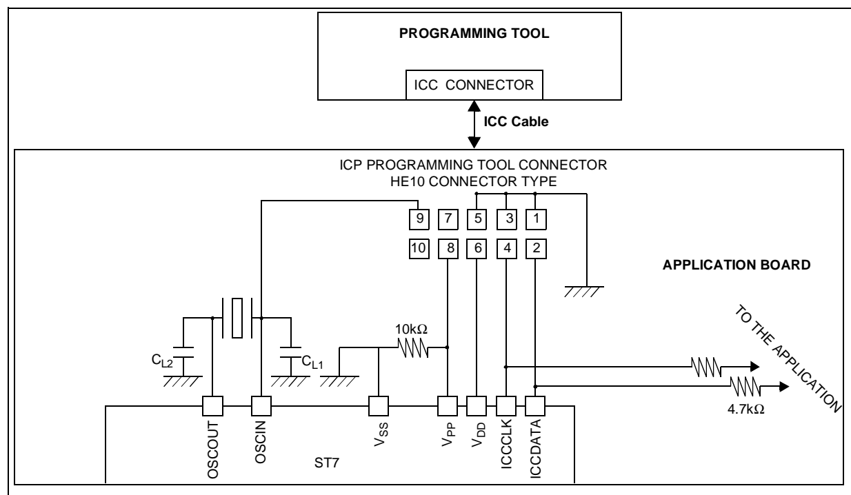
Figure 7. Typical ICP Interface
