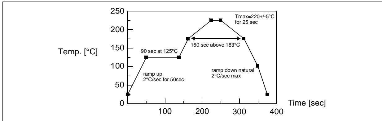
Figure 49. Recommended Reflow Oven Profile (MID JEDEC)
