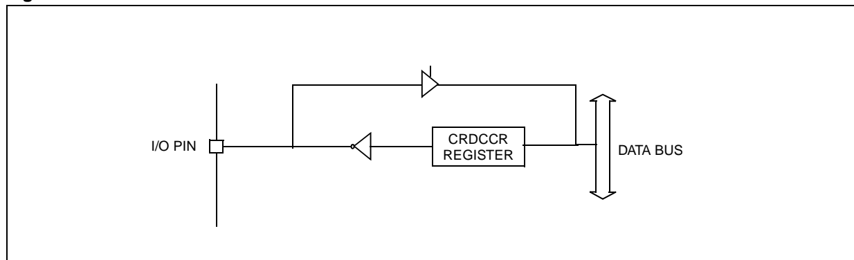
Figure 37. Smartcard I/O Pin Structure
