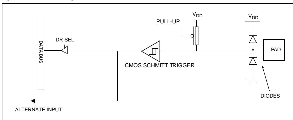
Figure 24. Port C Configuration
