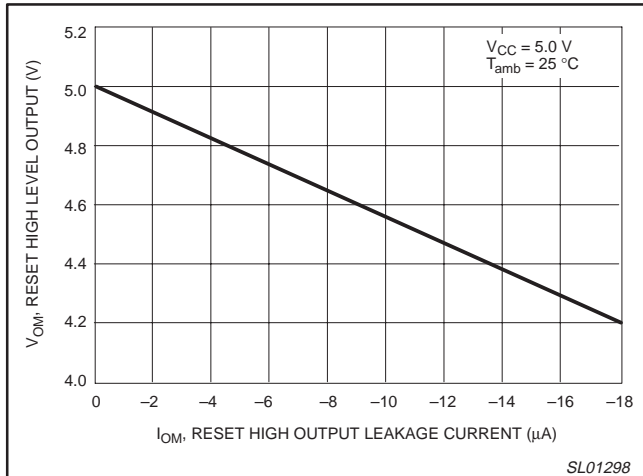
Figure 9. RESET HIGH-level voltage vs. current.
