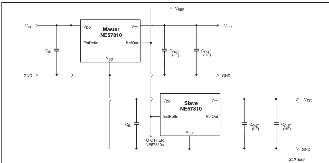
Figure 14. Cascading terminator systems for complex memory systems.
