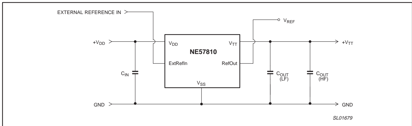
Figure 13. Externally programmed V_{TT} .
