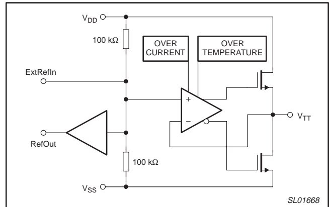
Figure 9. Block diagram.
