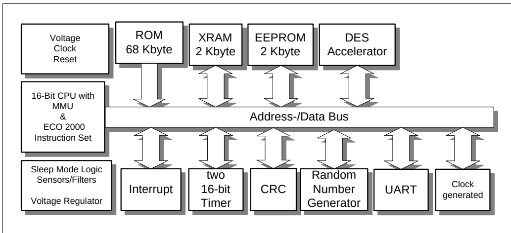
Figure 2: Block Diagram SLE 66C24PE
