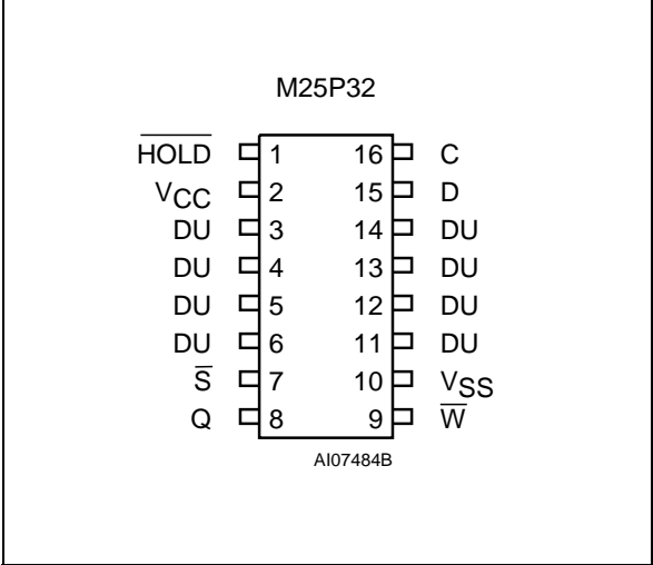
Figure 4. SO Connections
