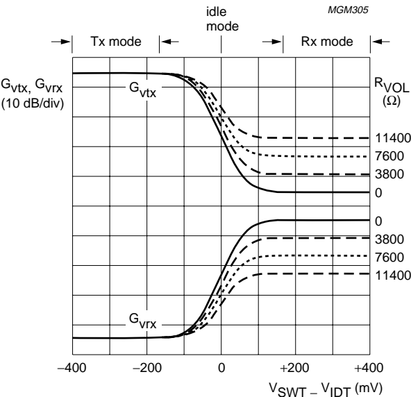
Fig.13 Switch-over behaviour.
