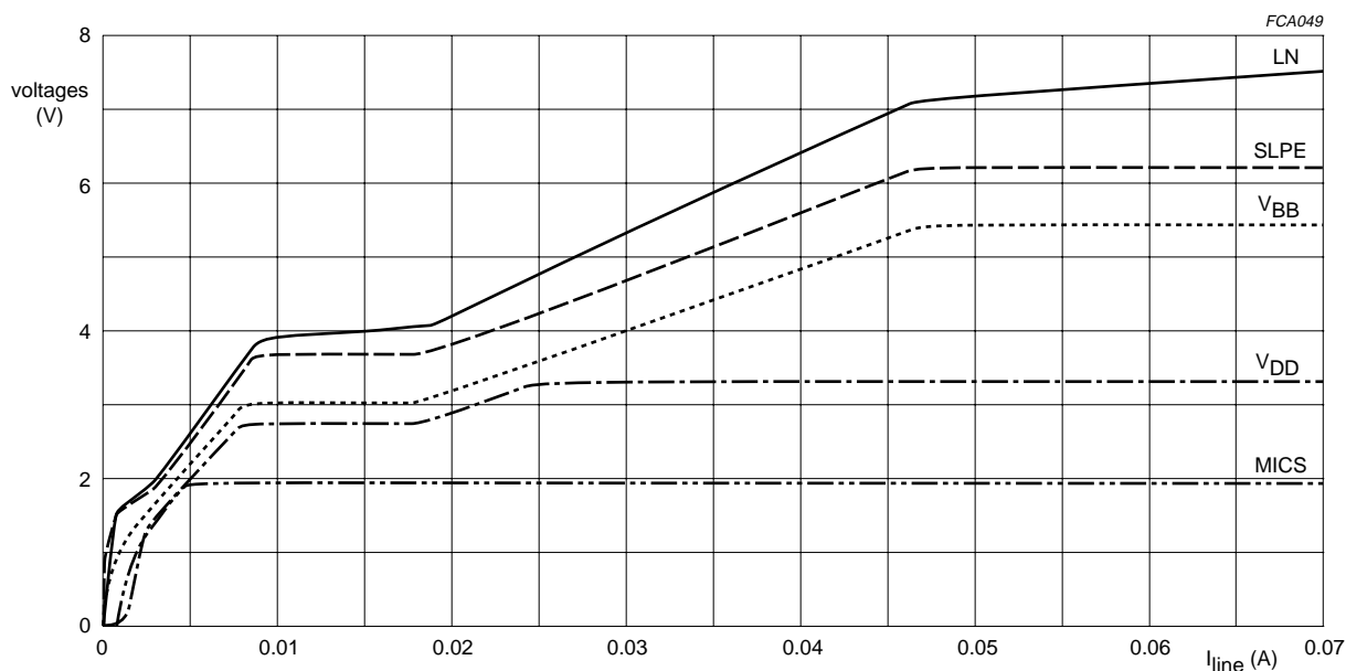
Fig.4 Main DC voltages.
