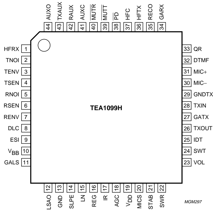
Fig.2 Pin configuration.
