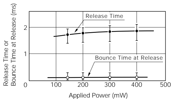
RELEASE TIME WITH DIODE
