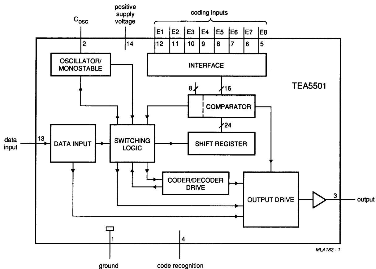
Fig.1 Block diagram.
