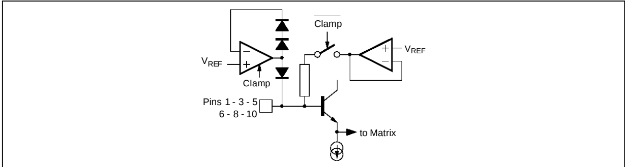
Figure 3 : Video OUT
