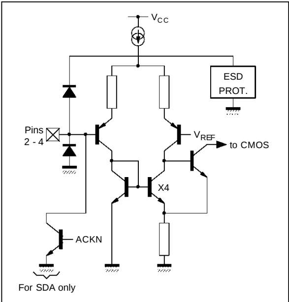
Figure 5 : Bus Inputs
