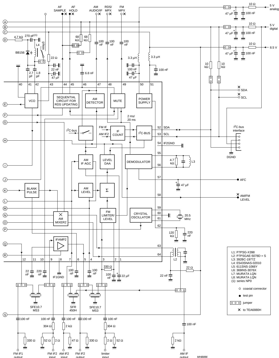
Fig.10 Test circuit (continued from Fig.9).
