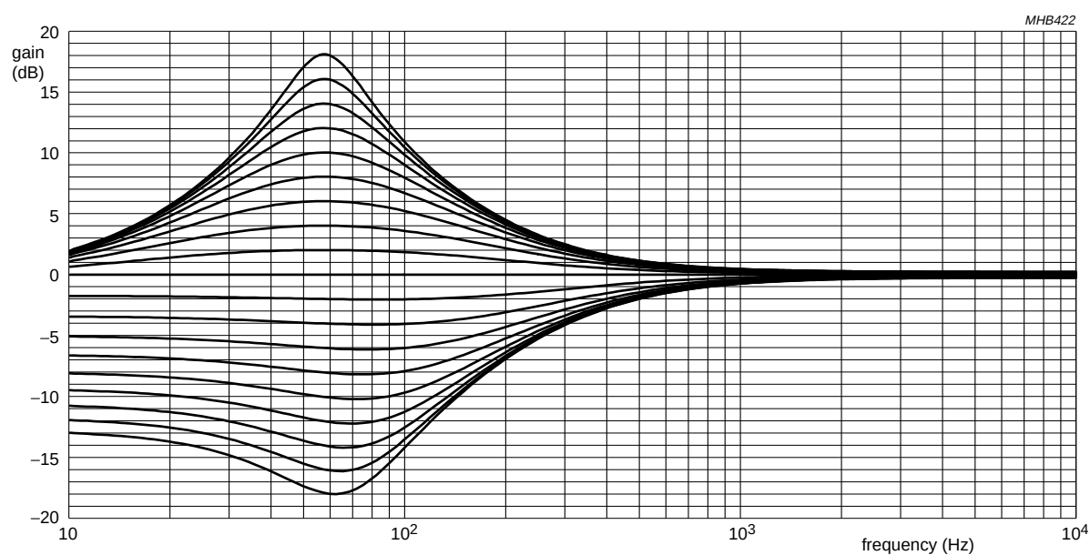
Fig.17 Bass curve with 2 \times 220 \text{ nF} and R = 3.3 \text{ k}\Omega external, BSYB = 1 for gain and BSYC = 0 for cut.
