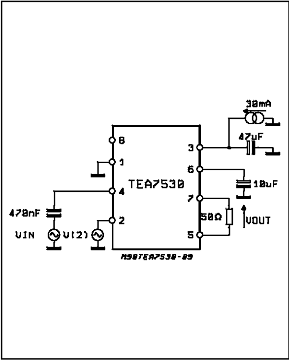
Figure 8: Anti-loading Feedback System at G = GATT
