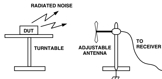
Figure 30. Radiated Emissions Test Setup
