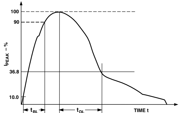
Figure 23. Human Body Model ESD Current Waveform
