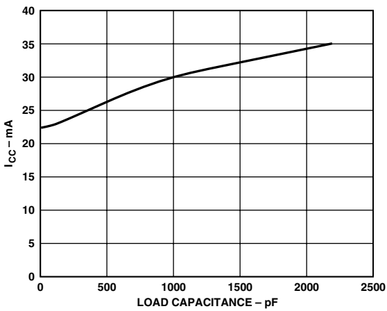
Figure 8. Supply Current vs. Load Capacitance ( R_L = 3\text{ k}\Omega )
