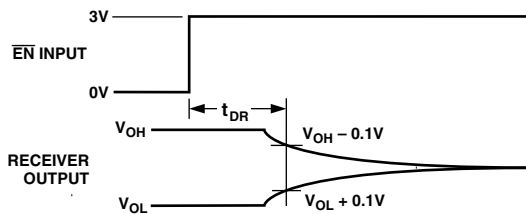
Figure 19. Receiver Disable Timing
