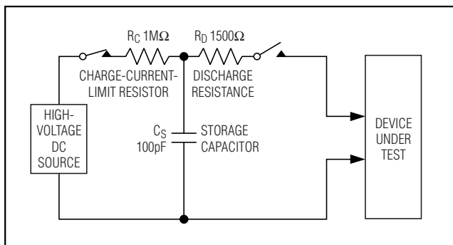
Figure 7a. Human Body ESD Test Model
