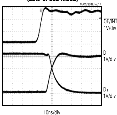
DRIVER DISABLE DELAY (LOW-SPEED MODE)
