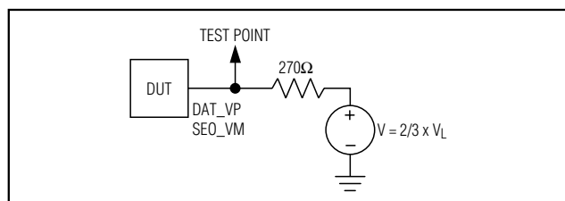
Figure 4. Load for DAT_VP, SEQ_VM Enable/Disable Time Measurements
