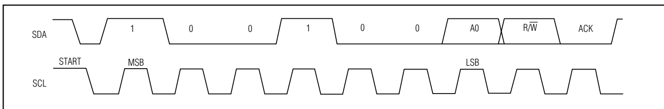
Figure 15. Slave Address
