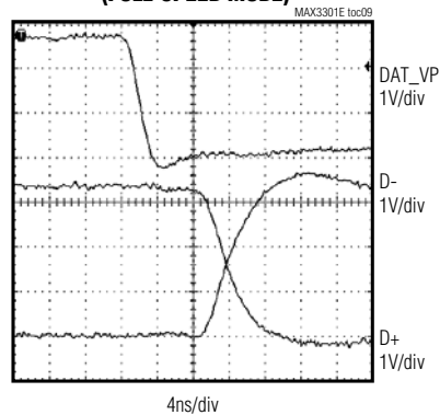
DRIVER PROPAGATION DELAY HIGH-TO-LOW (FULL-SPEED MODE)
