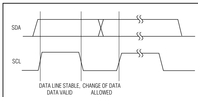
Figure 16. Bit Transfer
