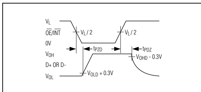
Figure 8. Enable and Disable Timing
