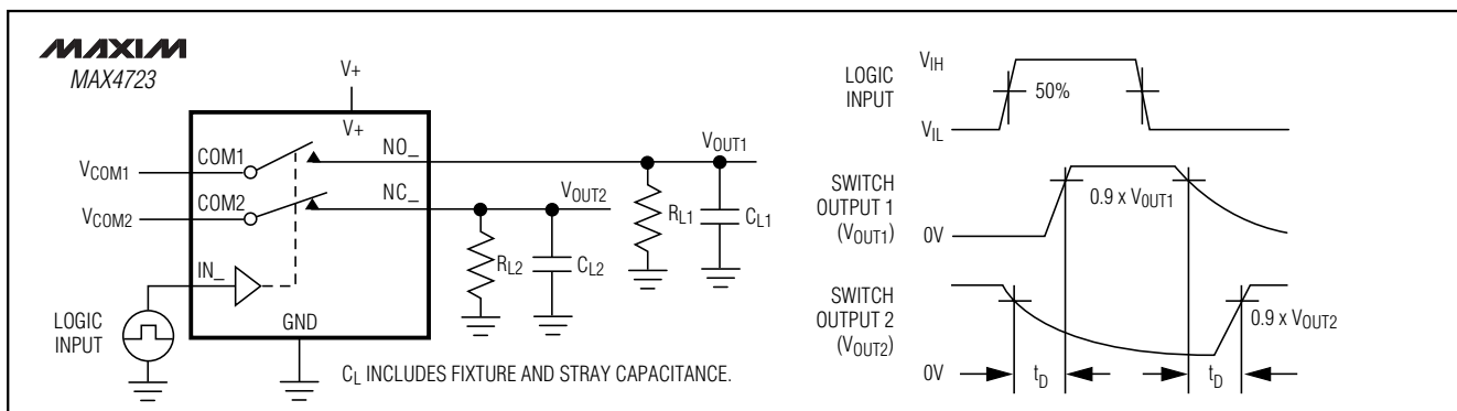
Figure 2. Break-Before-Make Interval
