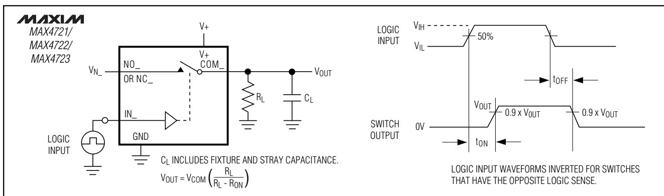
Figure 1. Switching Time
