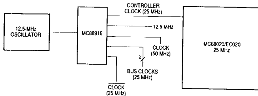
Figure 9-7. High-Resolution Clock Controller
