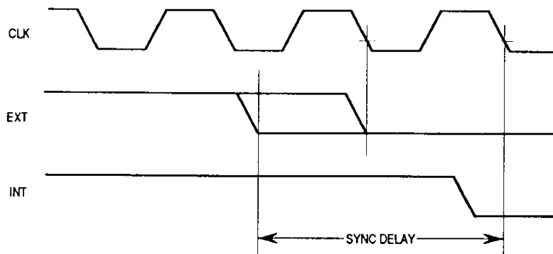
Figure 5-1. Relationship between External and Internal Signals
