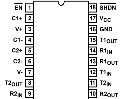
ICL3222E (PDIP, SOIC) TOP VIEW
