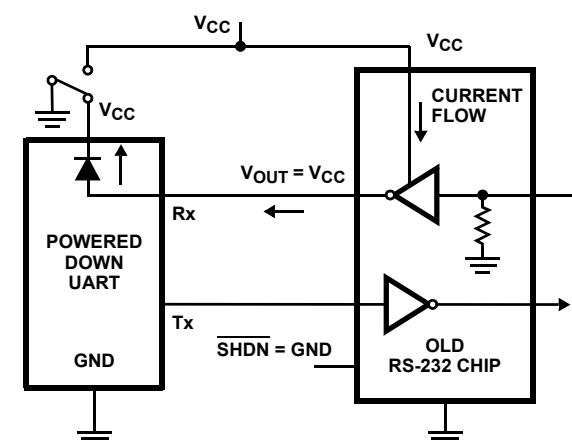
FIGURE 2. POWER DRAIN THROUGH POWERED DOWN PERIPHERAL
