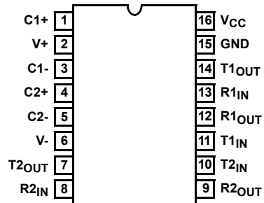
ICL3232E (SOIC, SSOP, TSSOP-16) TOP VIEW
