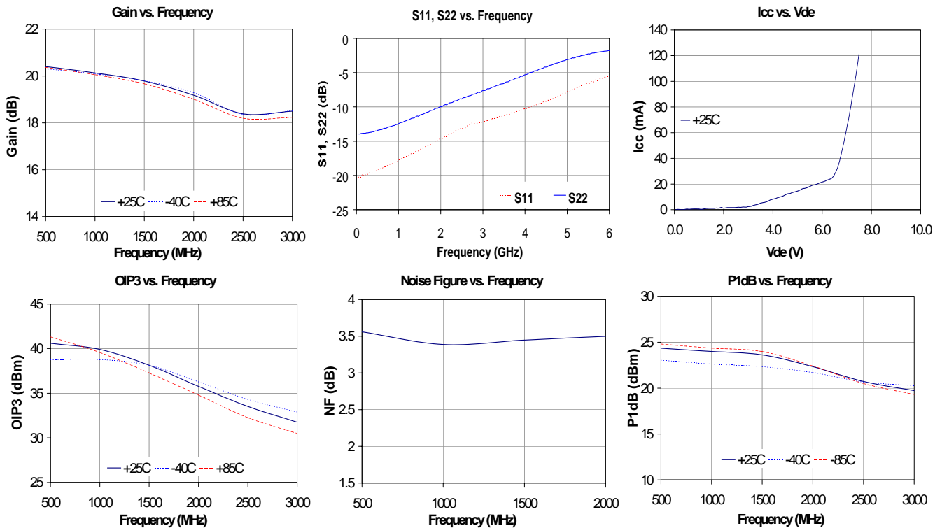
S-Parameters ( V_{device} = +7.2 \text{ V} , I_{cc} = 110 \text{ mA} , T = 25°C, calibrated to device leads)
