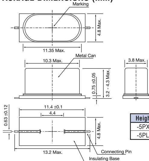
Figure 1) CSM-7X - Top, Side, Bottom and End views
