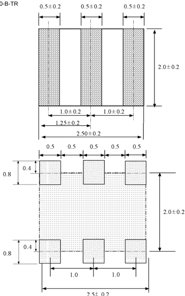
Figure 2) Bottom View & Suggested Land
