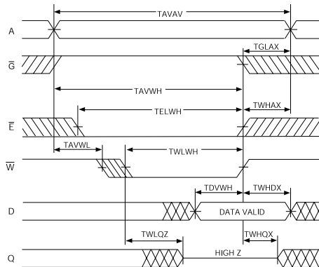
FIG. 6 WRITE CYCLE 1 - \bar{W} CONTROLLED
