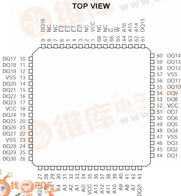
FIG. 1 PIN CONFIGURATION
