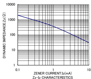
Z Z -I Z CHARACTERISTICS
