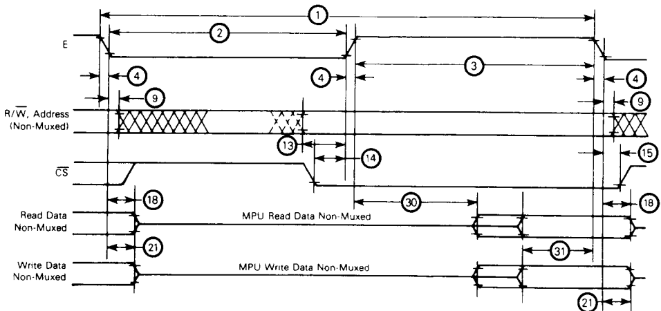
FIGURE 1 — BUS TIMING
