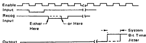
FIGURE 11 — INPUT JITTER
