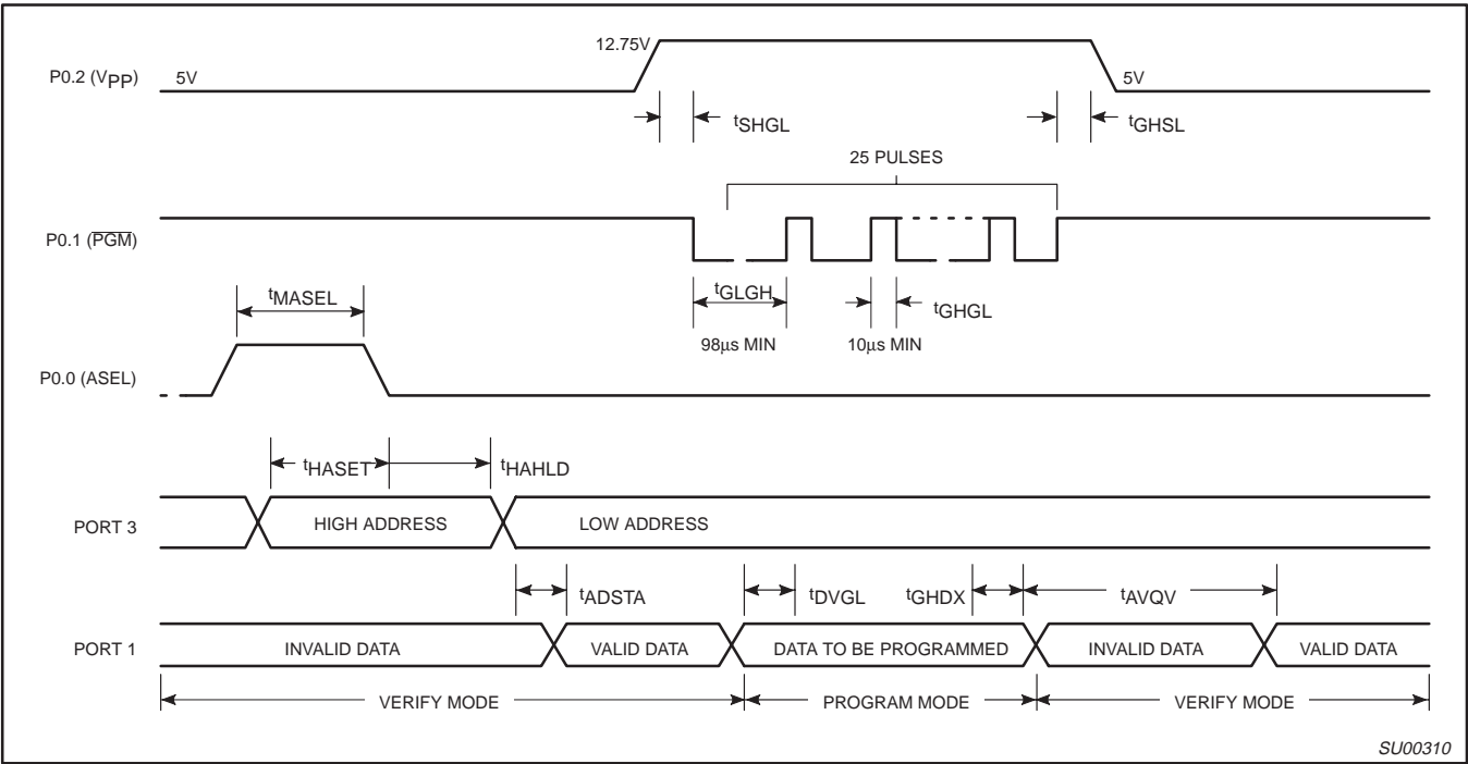
Figure 6. Program/Verify Cycle
