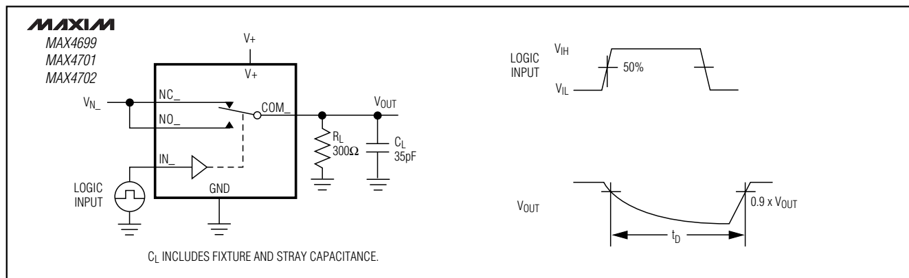
Figure 3. Break-Before-Make Interval
