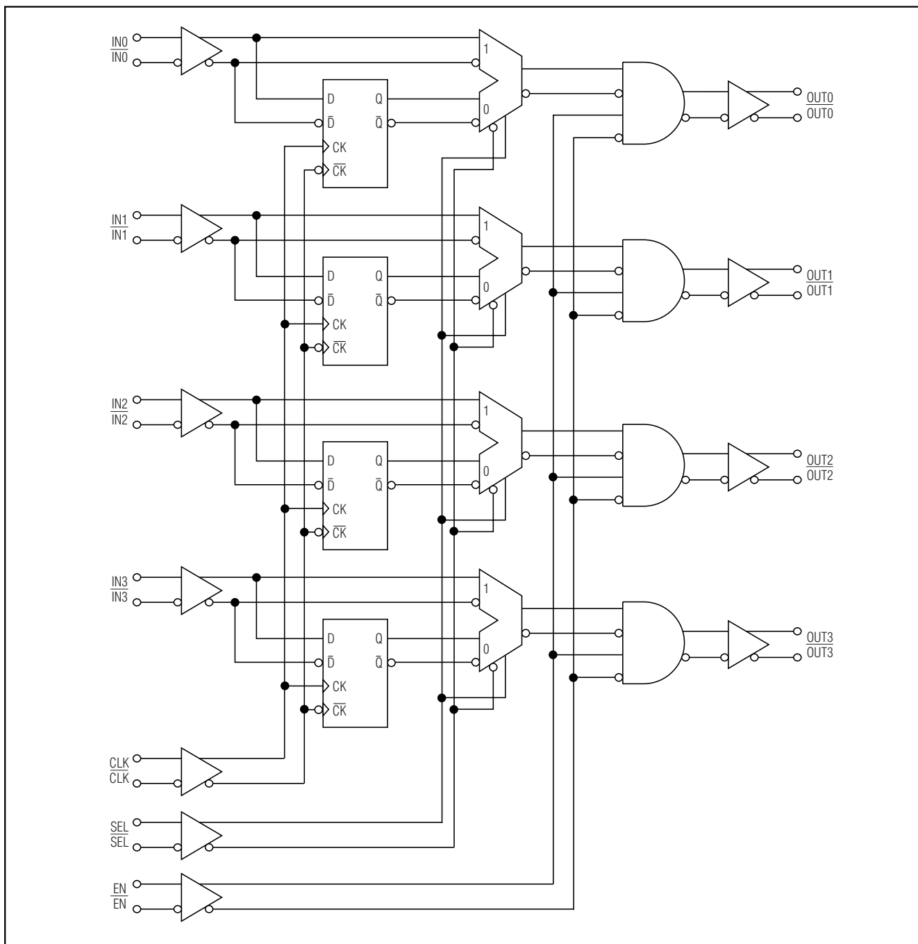
Functional Diagram
