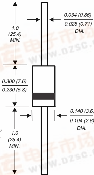
DO-204AC
