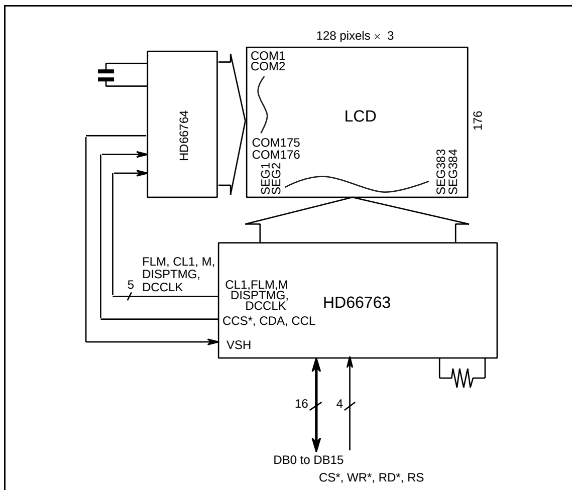
Figure 8 System Configuration
