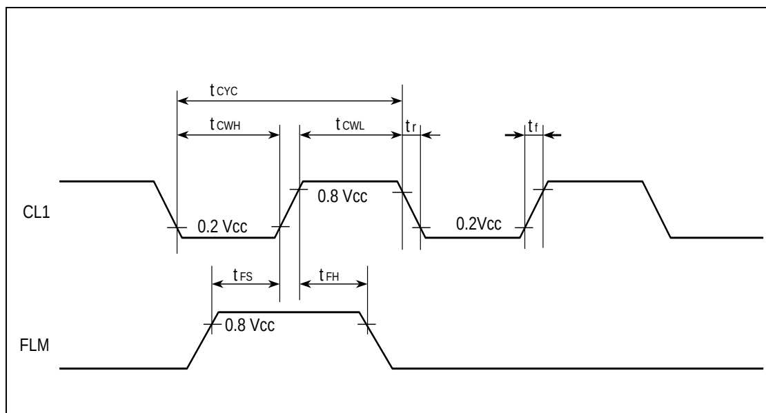
Figure 14 LCD control signal Timing
