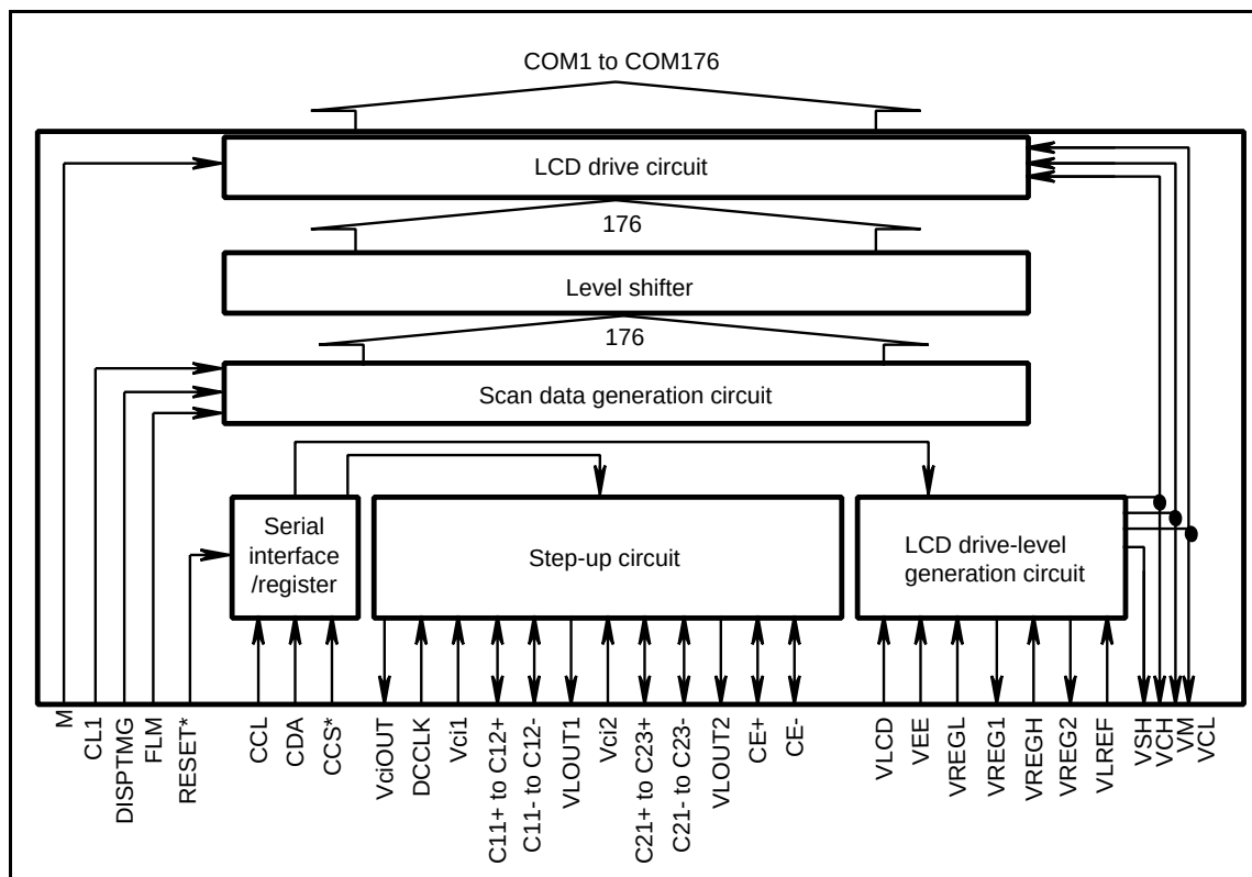
Figure 1 Block Diagram
