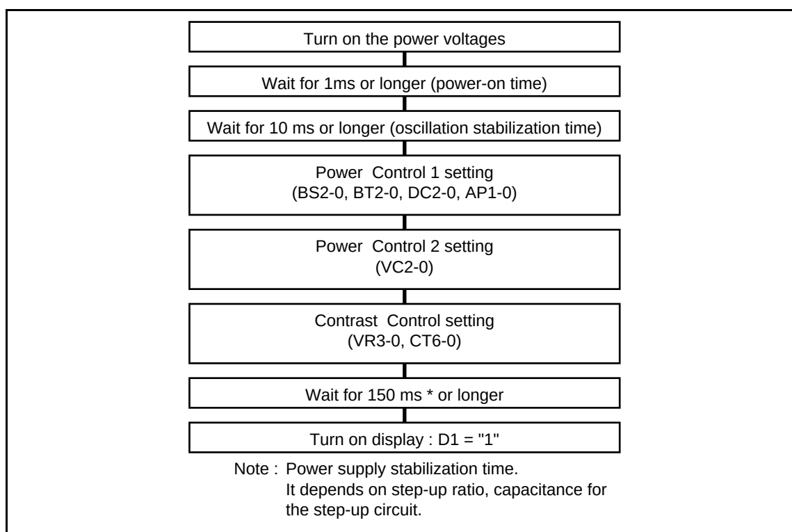
Figure 12 Power-on Sequence
