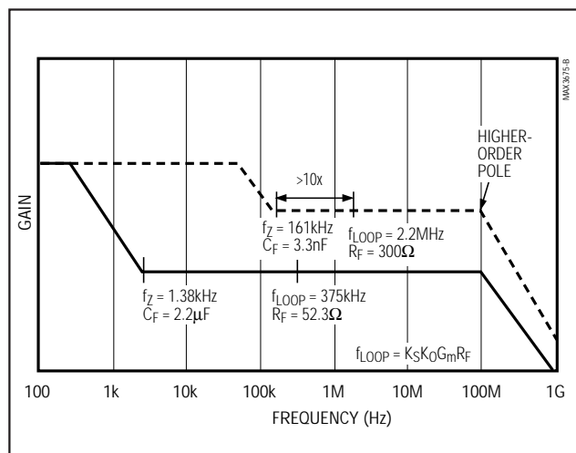
Figure 3. Loop-Filter Response
