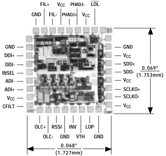
Chip Topography
