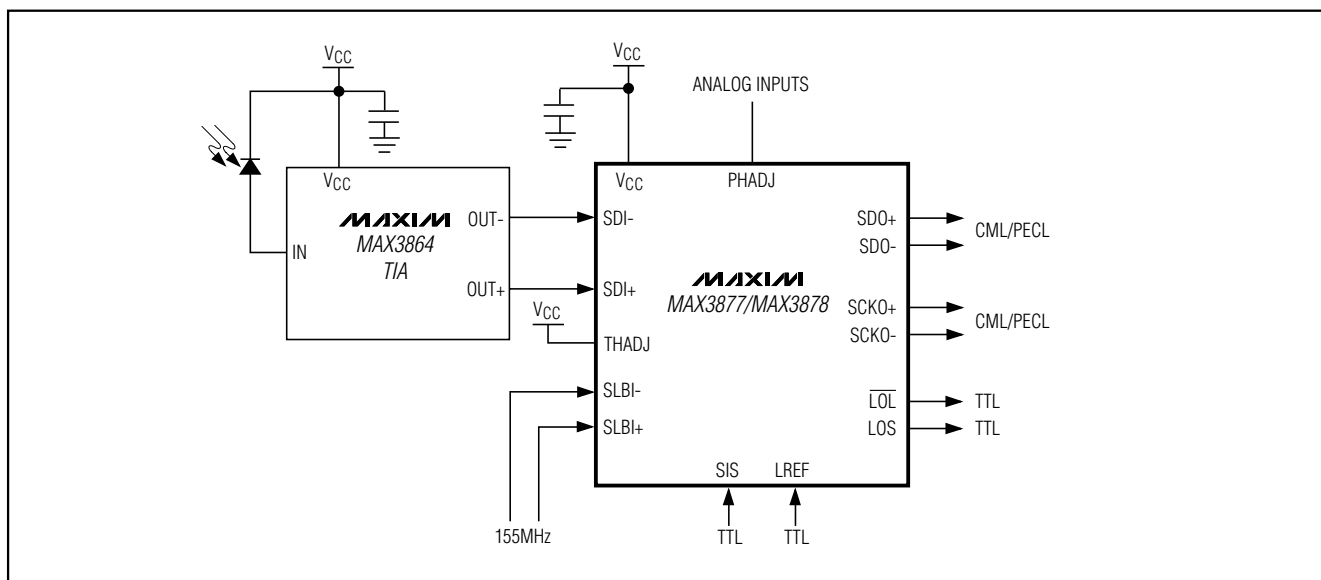
Figure 12. Typical Application Circuit (Interfacing with the MAX3864 TIA without using threshold adjust)
