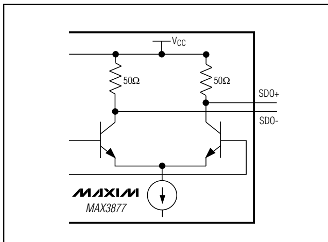
Figure 11. CML Outputs
