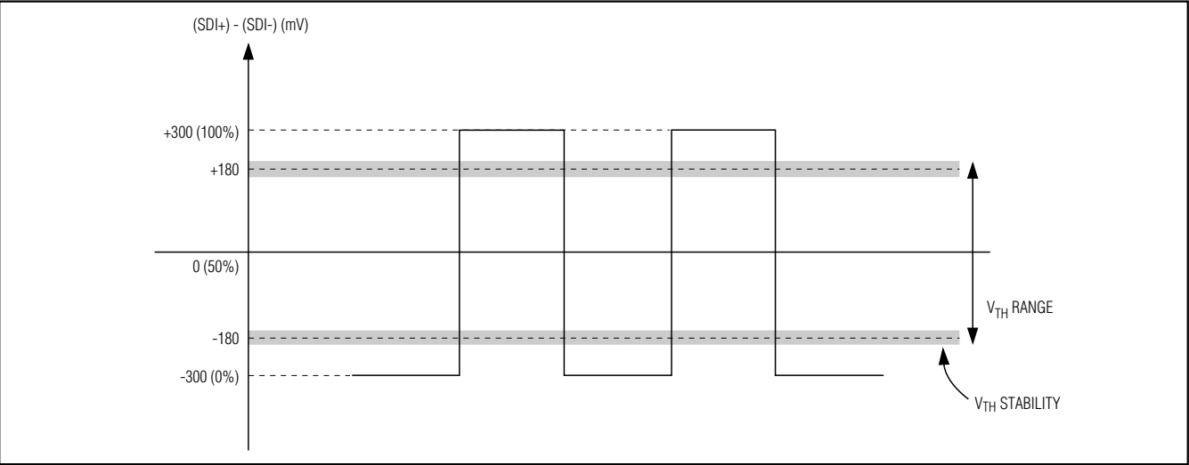
Figure 3. Definition of Input Threshold
