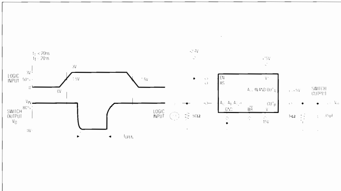
Figure 4. Opn Time (B.B.M.) Interval Test Circuit
