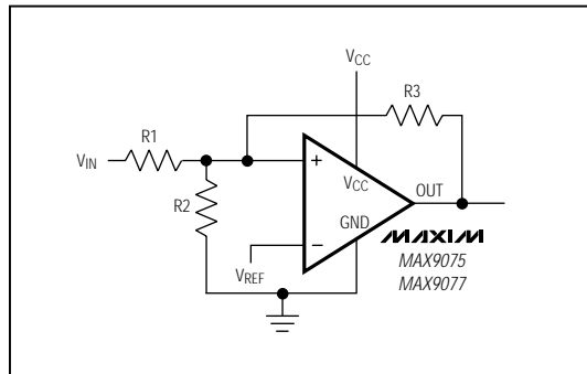
Figure 1. Adding Hysteresis
