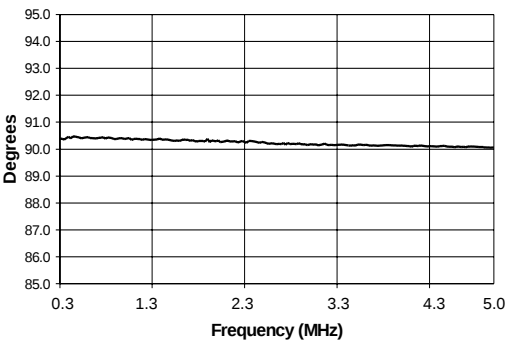
Phase Unbalance
