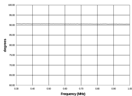
Phase Unbalance
