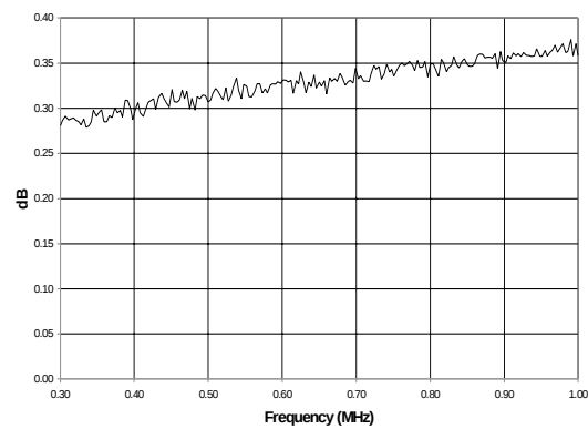
Amplitude Unbalance
