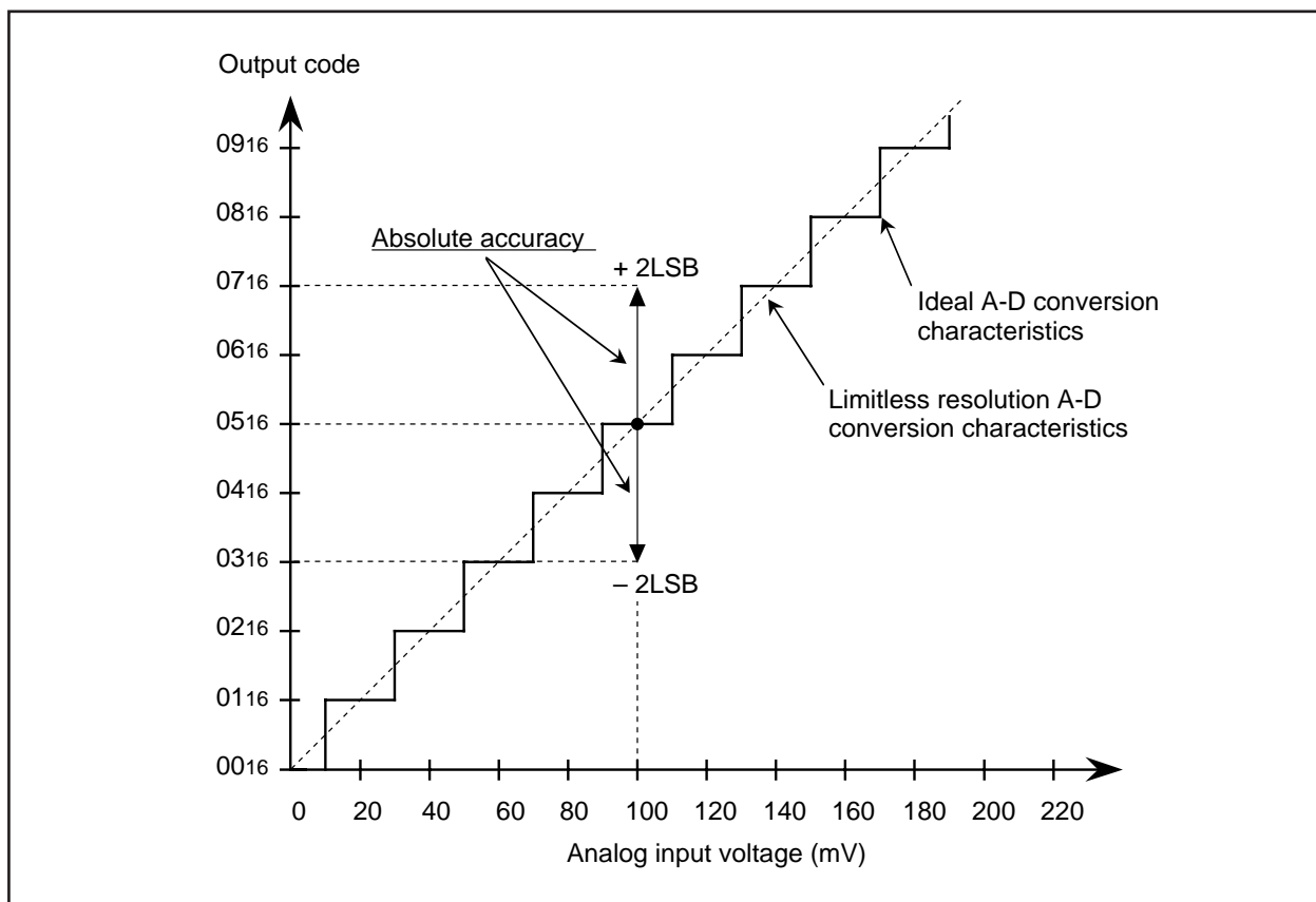
Fig. 12.8.4 Definition of A-D Conversion Accuracy
