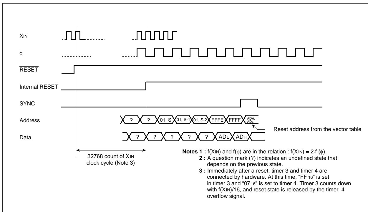
Fig.14.2 Reset Sequence
