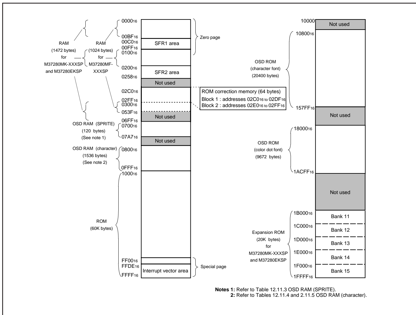
Fig. 12.2.1 Memory Map
