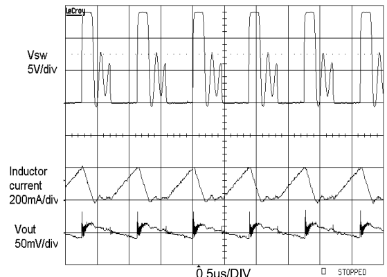
Vsw, I L , & Vout Signal Waveforms
