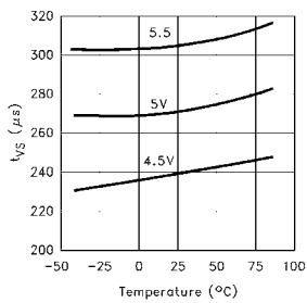
Vertical Sync Pulse Width RSET = 681k
