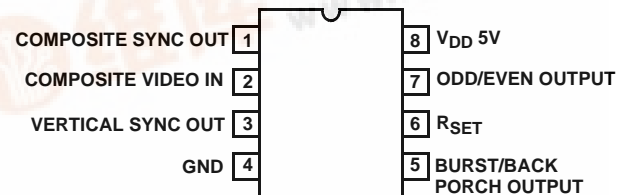
EL1882C (8-PIN PDIP, SO) TOP VIEW
