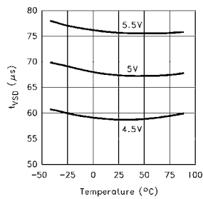
Composite Sync to Odd/Even Delay Time RSET = 681k
