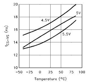
Composite Sync vs Delay Time RSET = 681k
