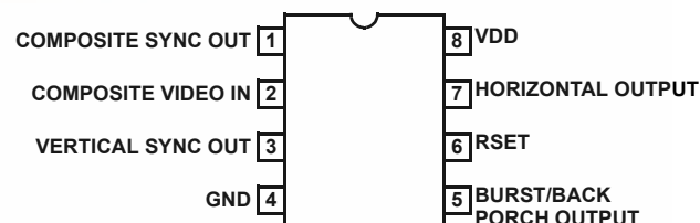
EL1883 (8-PIN SO) TOP VIEW
