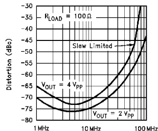
3rd Harmonic Distortion
