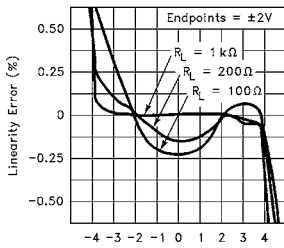
Integral Linearity Error
