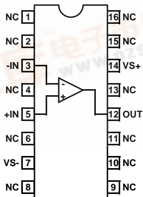
EL2160 [16-PIN SO (0.300")] TOP VIEW
