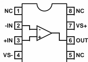
EL2160 (8-PIN PDIP, SO) TOP VIEW
